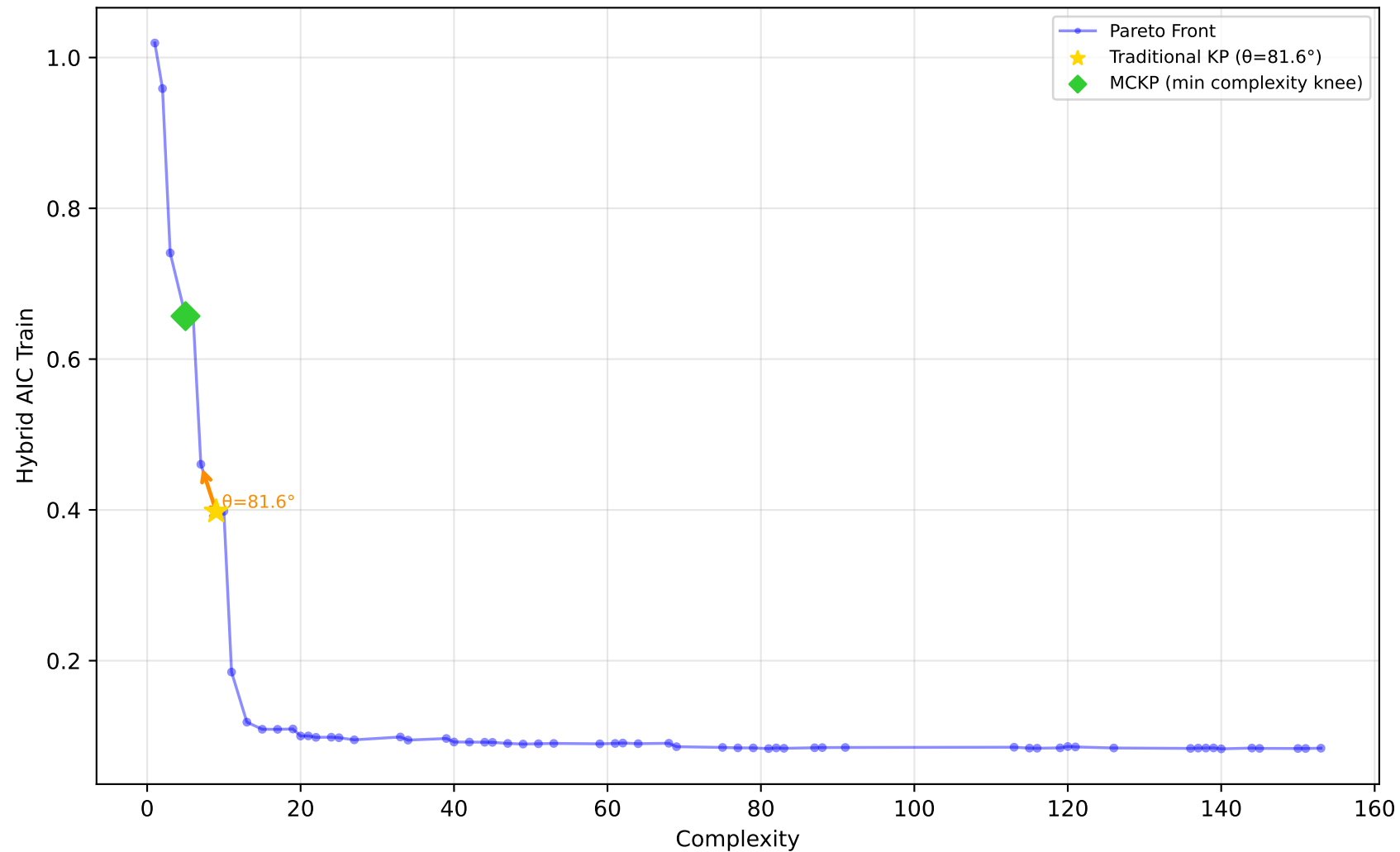
529_pollen - Run 13 - SVP - Hybrid AIC Train \lambda_1=0.60, \lambda_2=0.40, \lambda_3=1.00 | Difficulty: 1.00 | Method: hmr
