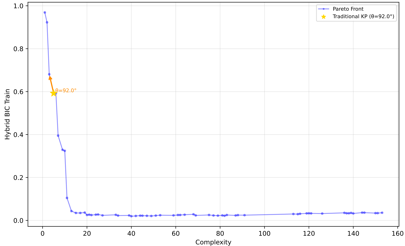
529_pollen - Run 13 - SVP - Hybrid BIC Train \lambda_1=0.10, \lambda_2=0.80, \lambda_3=0.30 | Difficulty: 1.00 | Method: hmr
