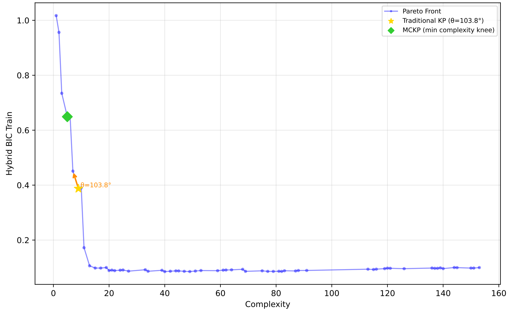
529_pollen - Run 13 - SVP - Hybrid BIC Train \lambda_1=0.60, \lambda_2=0.40, \lambda_3=1.00 | Difficulty: 1.00 | Method: hmr
