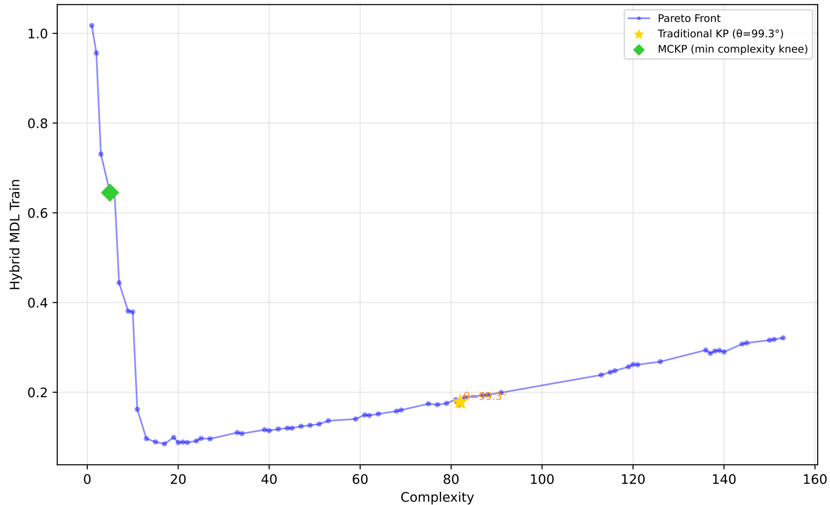
529_pollen - Run 13 - SVP - Hybrid MDL Train \lambda_1=0.60, \lambda_2=0.40, \lambda_3=1.00 | Difficulty: 1.00 | Method: hmr
