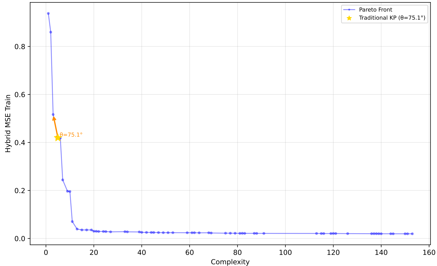
529_pollen - Run 13 - SVP - Hybrid MSE Train \lambda_1=0.10, \lambda_2=0.80, \lambda_3=0.30 | Difficulty: 1.00 | Method: hmr
