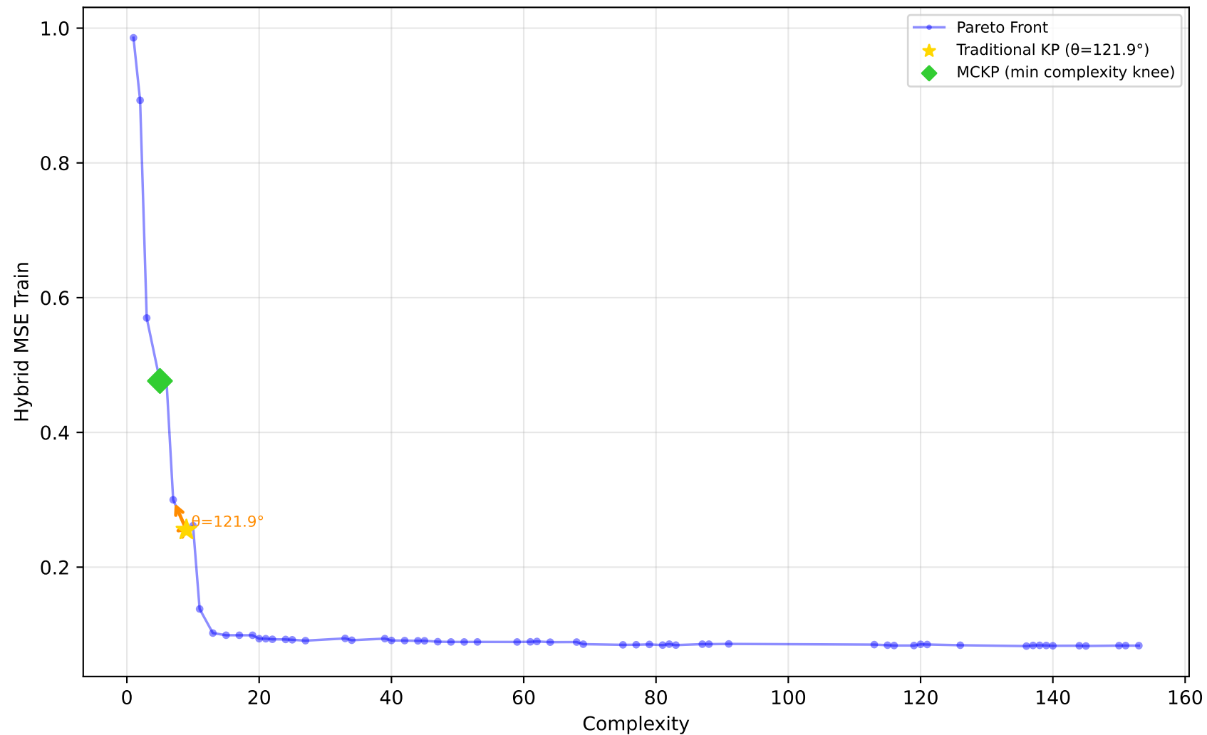
529_pollen - Run 13 - SVP - Hybrid MSE Train \lambda_1=0.60, \lambda_2=0.40, \lambda_3=1.00 | Difficulty: 1.00 | Method: hmr
