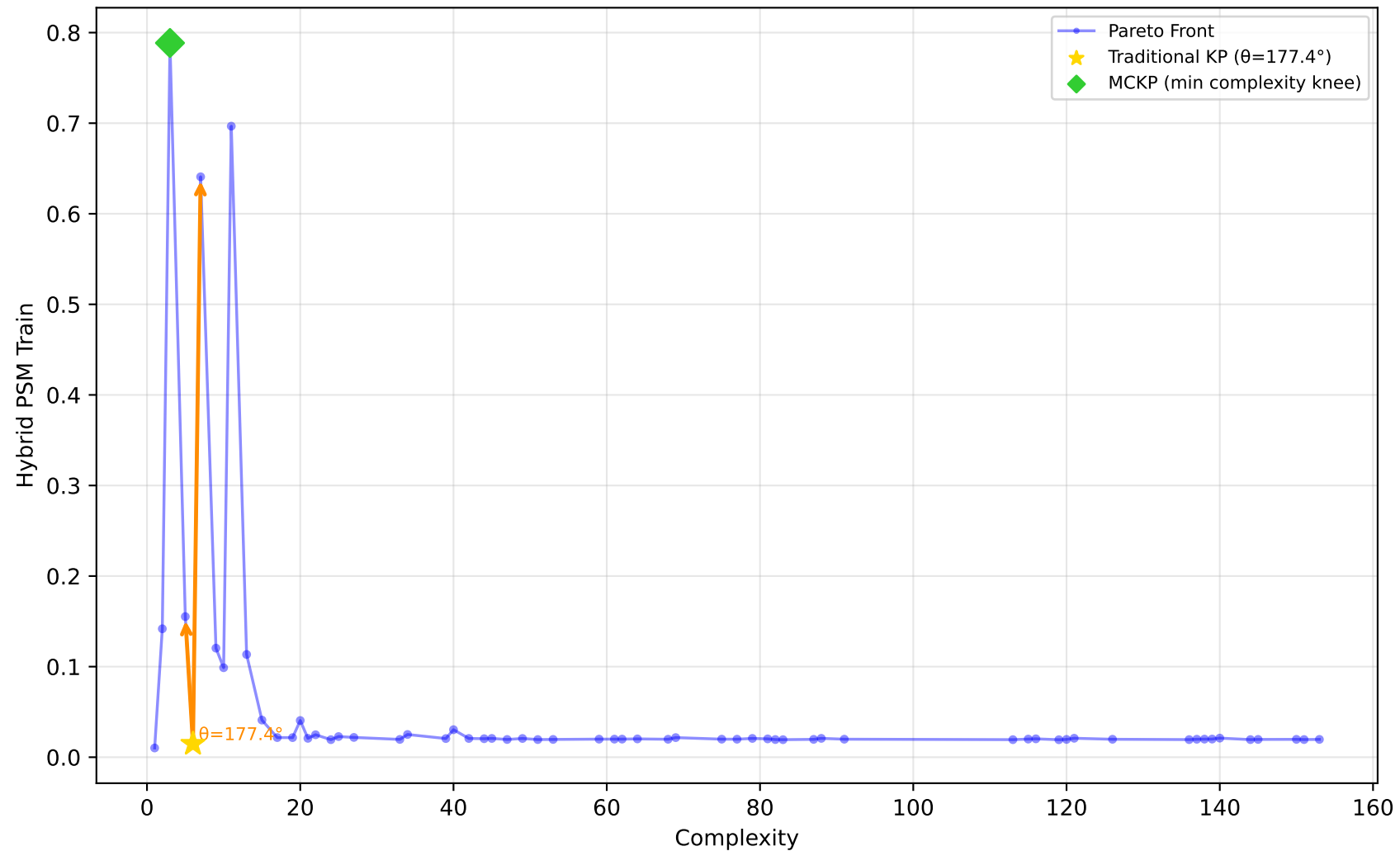
529_pollen - Run 13 - SVP - Hybrid PSM Train \lambda_1=0.10, \lambda_2=0.80, \lambda_3=0.30 | Difficulty: 1.00 | Method: hmr
