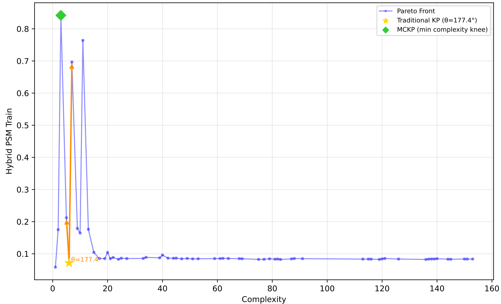
529_pollen - Run 13 - SVP - Hybrid PSM Train \lambda_1=0.60, \lambda_2=0.40, \lambda_3=1.00 | Difficulty: 1.00 | Method: hmr
