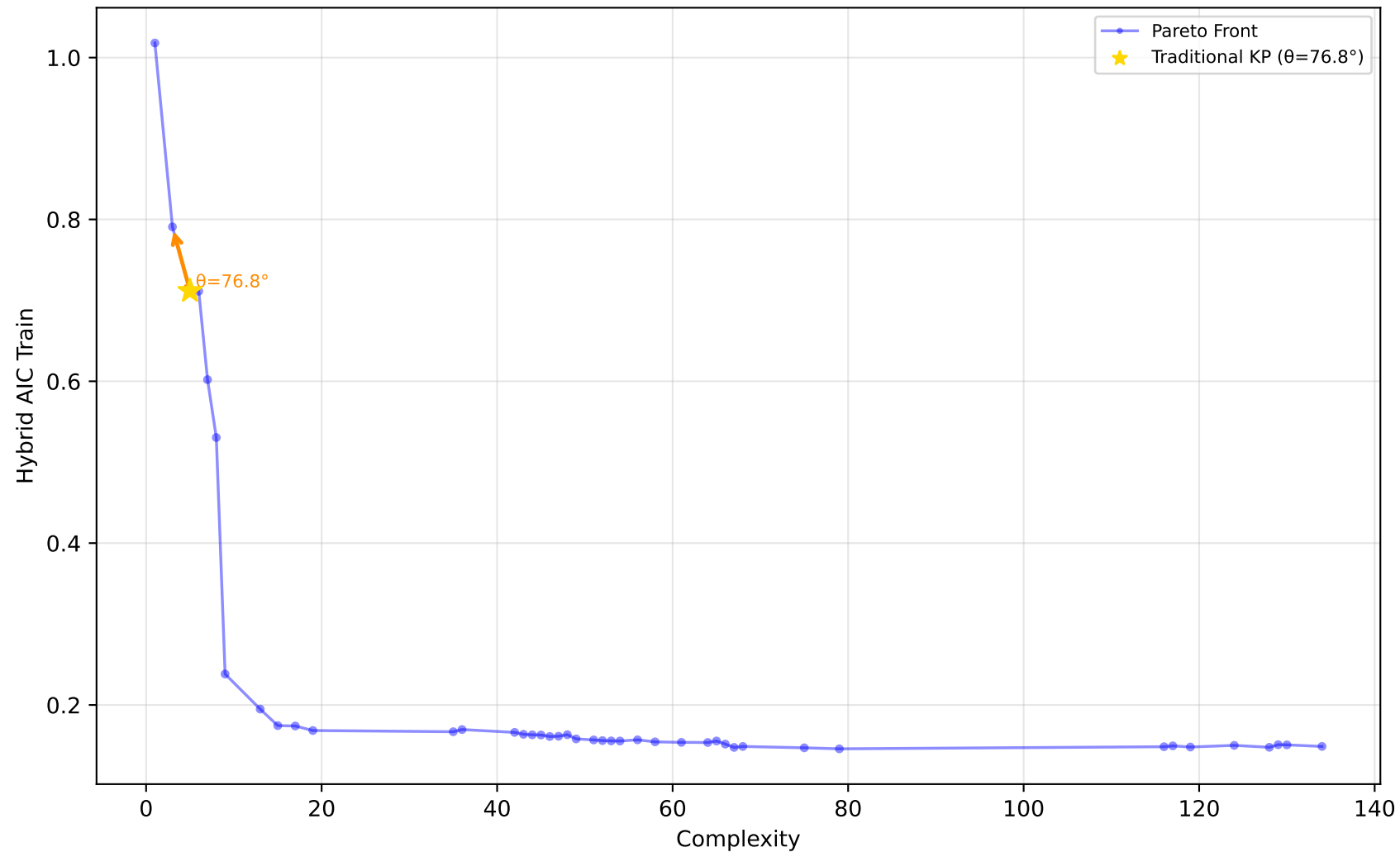
529_pollen - Run 14 - MVP - Hybrid AIC Train \lambda_1=0.90, \lambda_2=0.00, \lambda_3=0.00 | Difficulty: 1.00 | Method: hmr
