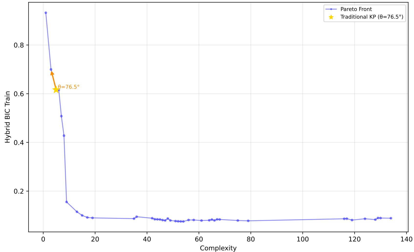
529_pollen - Run 14 - MVP - Hybrid BIC Train \lambda_1=0.00, \lambda_2=1.00, \lambda_3=0.80 | Difficulty: 1.00 | Method: hmr
