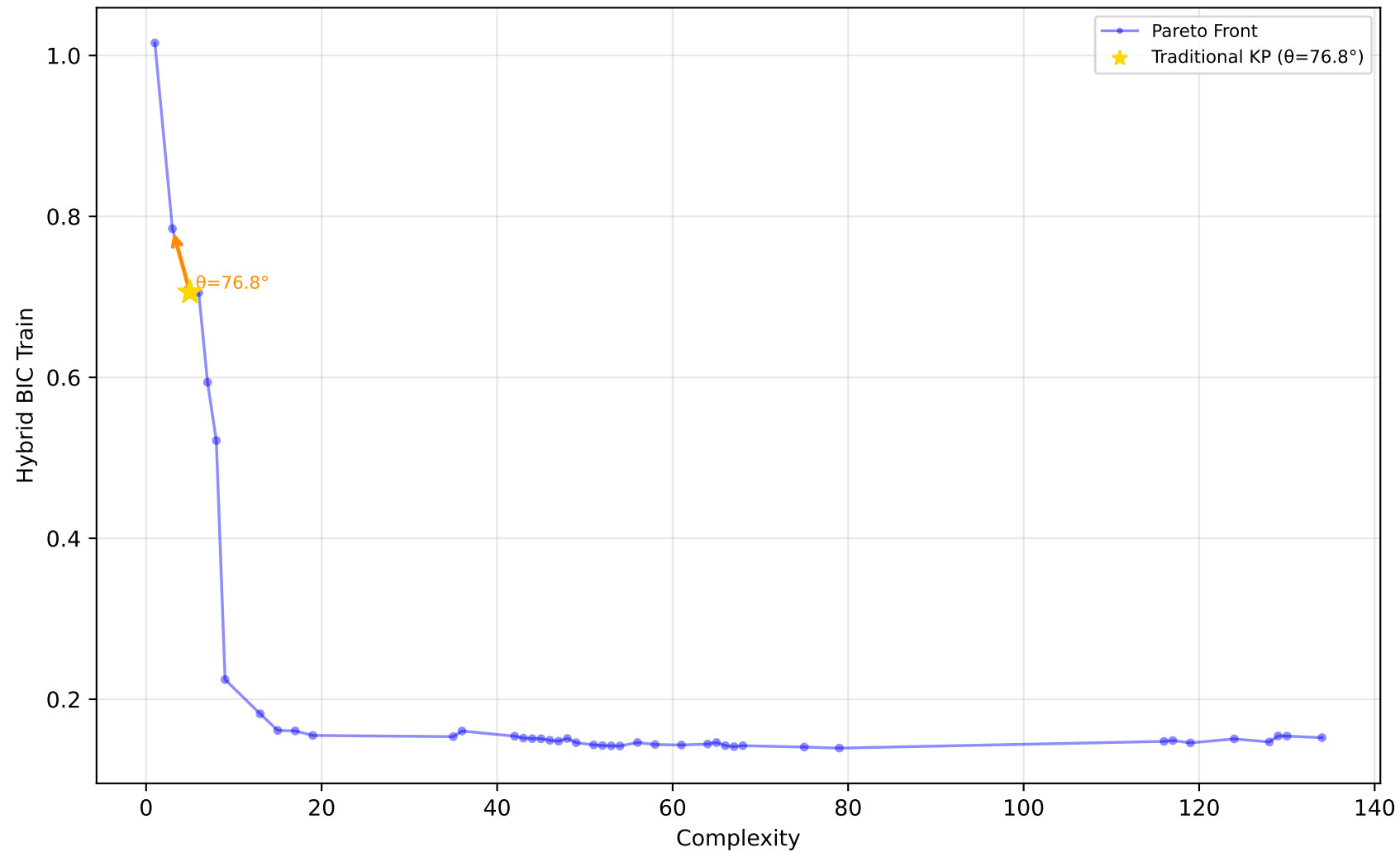
529_pollen - Run 14 - MVP - Hybrid BIC Train \lambda_1=0.90, \lambda_2=0.00, \lambda_3=0.00 | Difficulty: 1.00 | Method: hmr
