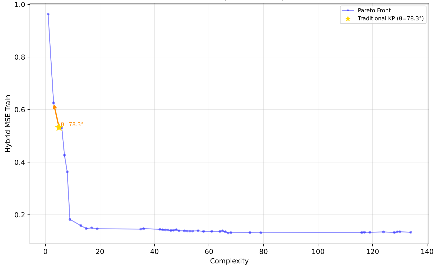
529_pollen - Run 14 - MVP - Hybrid MSE Train \lambda_1=0.90, \lambda_2=0.00, \lambda_3=0.00 | Difficulty: 1.00 | Method: hmr
