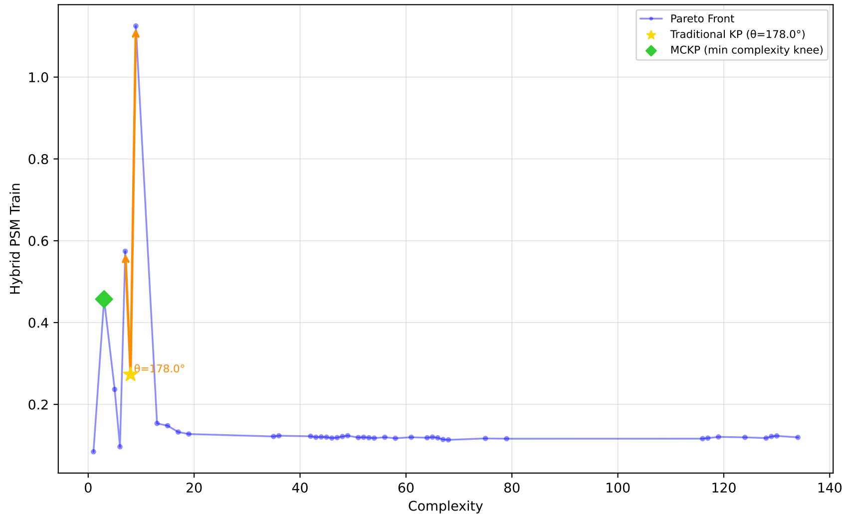
529_pollen - Run 14 - MVP - Hybrid PSM Train \lambda_1=0.90, \lambda_2=0.00, \lambda_3=0.00 | Difficulty: 1.00 | Method: hmr
