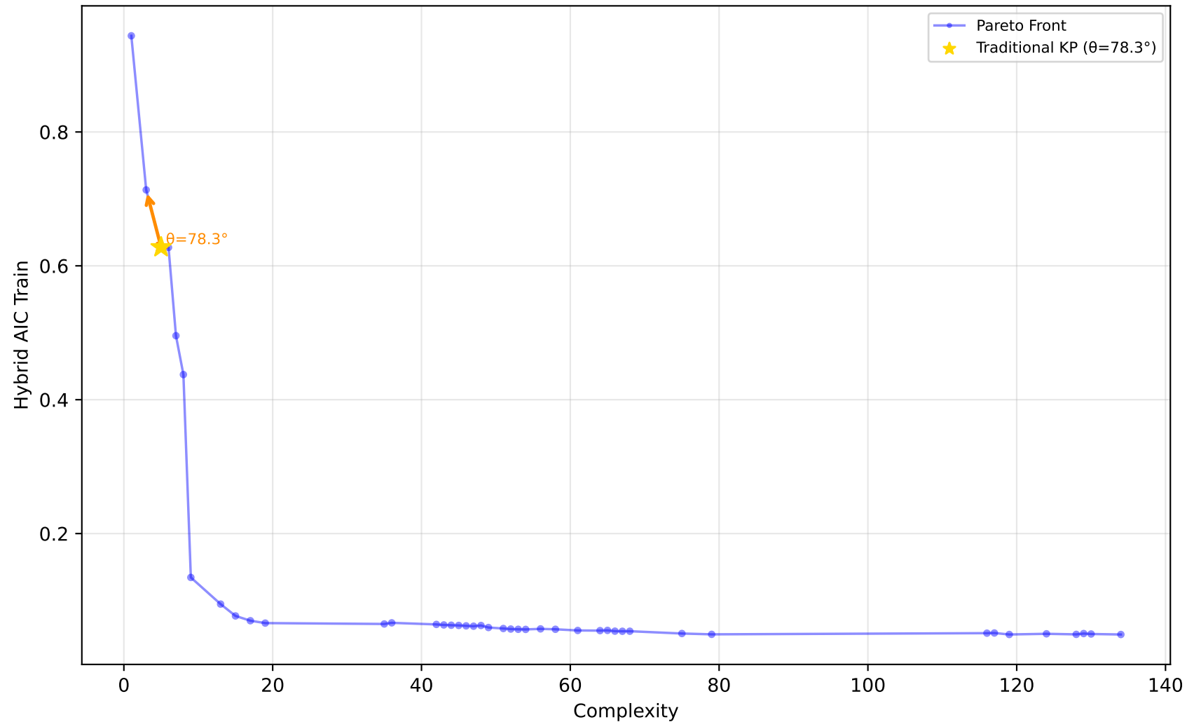
529_pollen - Run 14 - SVP - Hybrid AIC Train \lambda_1=0.10, \lambda_2=0.80, \lambda_3=0.30 | Difficulty: 1.00 | Method: hmr
