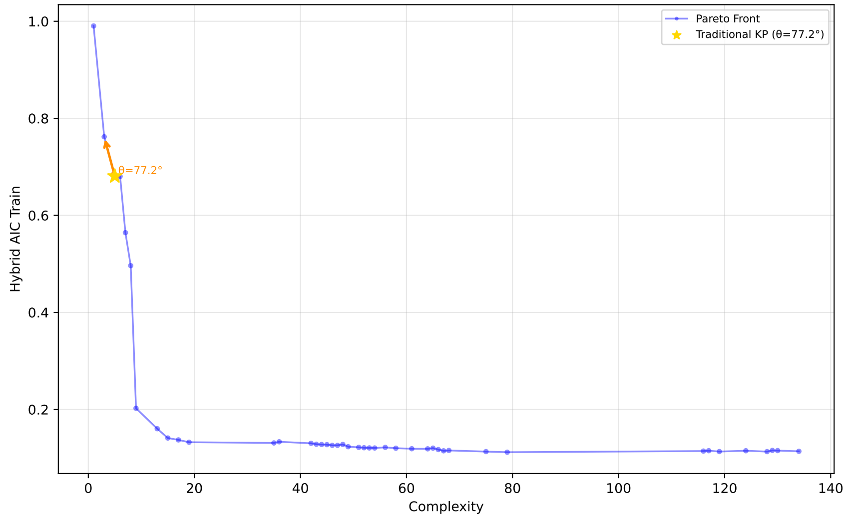
529_pollen - Run 14 - SVP - Hybrid AIC Train \lambda_1=0.60, \lambda_2=0.40, \lambda_3=1.00 | Difficulty: 1.00 | Method: hmr
