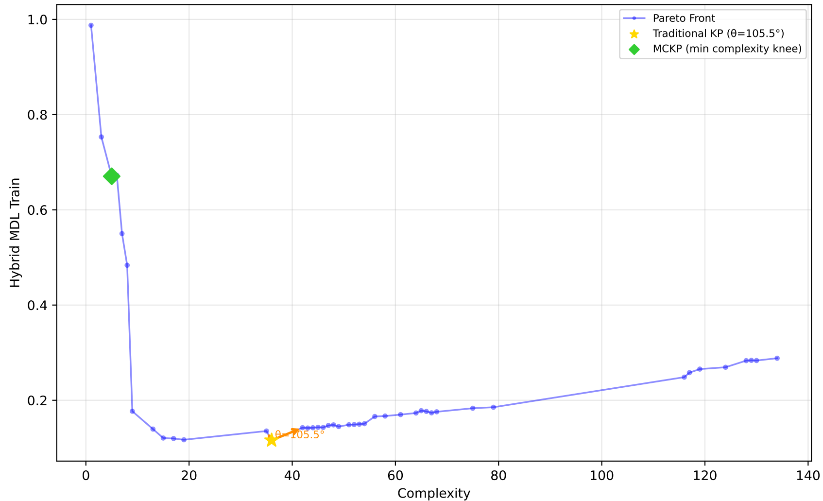
529_pollen - Run 14 - SVP - Hybrid MDL Train \lambda_1=0.60, \lambda_2=0.40, \lambda_3=1.00 | Difficulty: 1.00 | Method: hmr
