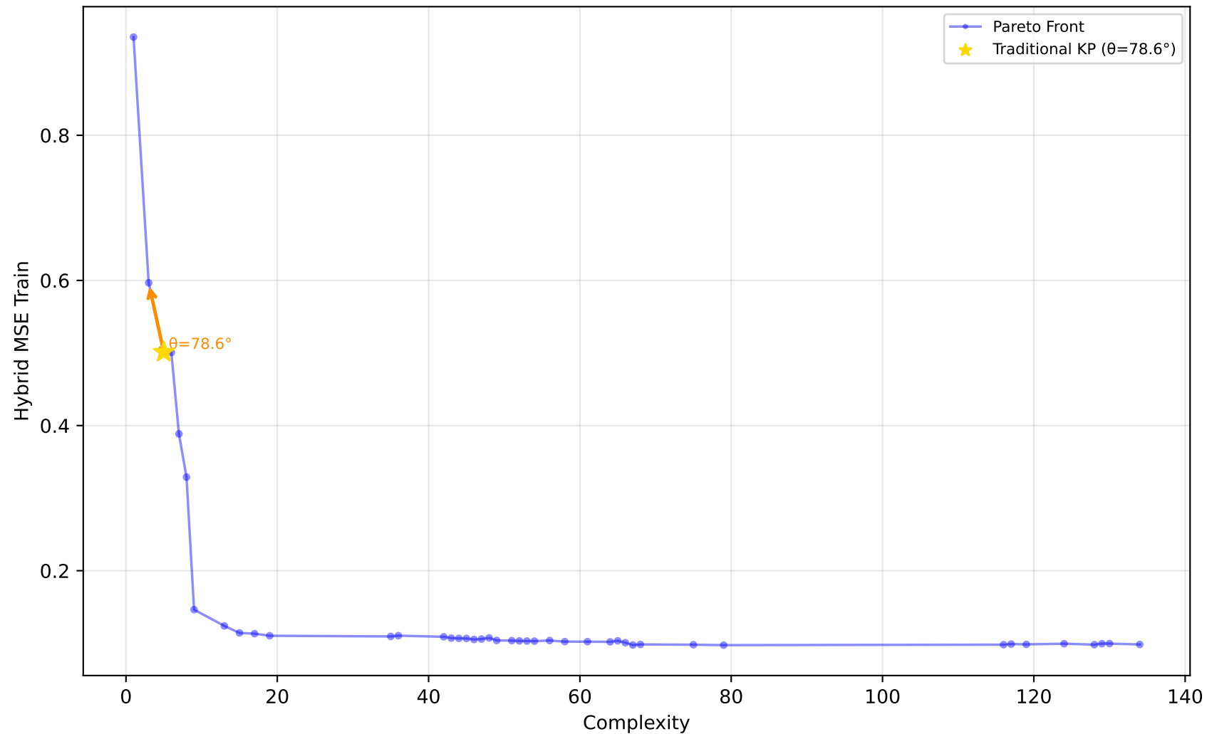
529_pollen - Run 14 - SVP - Hybrid MSE Train \lambda_1=0.60, \lambda_2=0.40, \lambda_3=1.00 | Difficulty: 1.00 | Method: hmr
