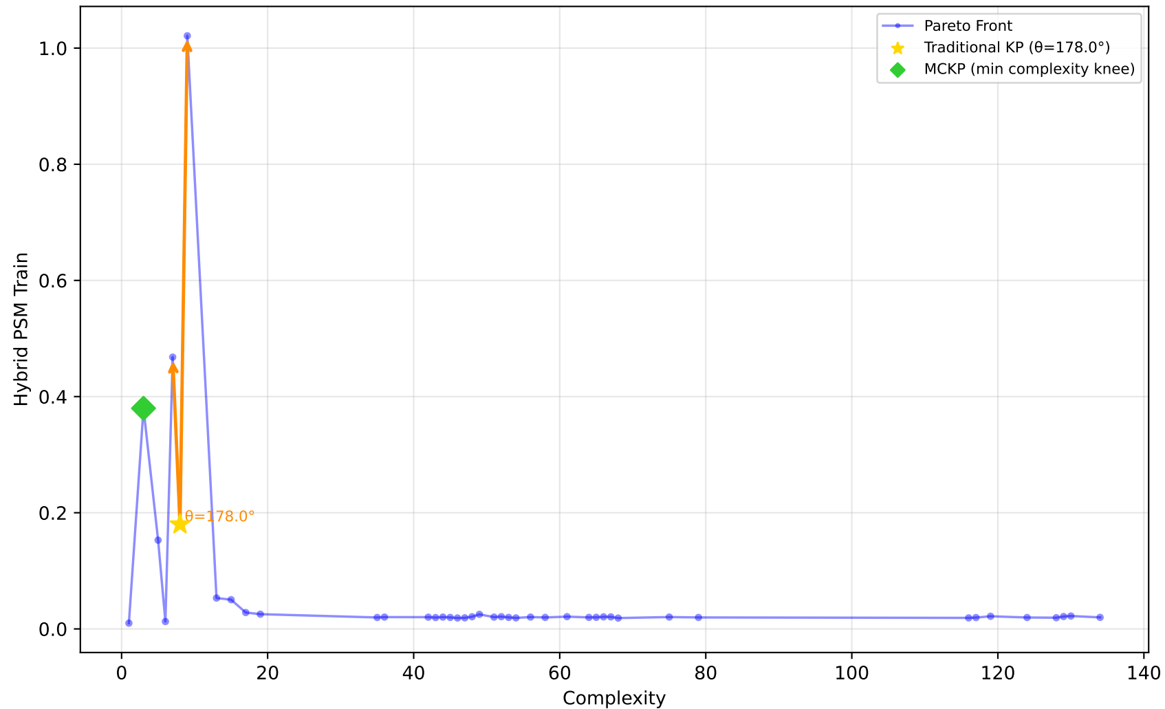
529_pollen - Run 14 - SVP - Hybrid PSM Train \lambda_1=0.10, \lambda_2=0.80, \lambda_3=0.30 | Difficulty: 1.00 | Method: hmr
