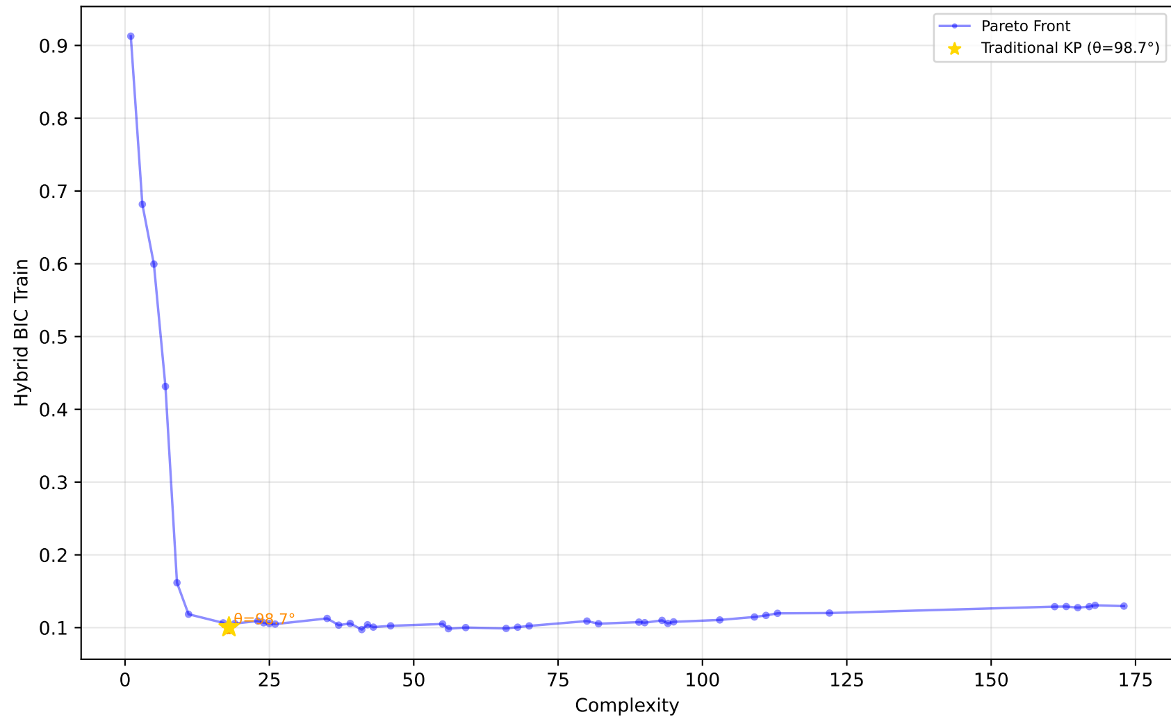
529_pollen - Run 15 - MVP - Hybrid BIC Train \lambda_1=0.00, \lambda_2=1.00, \lambda_3=0.80 | Difficulty: 1.00 | Method: hmr
