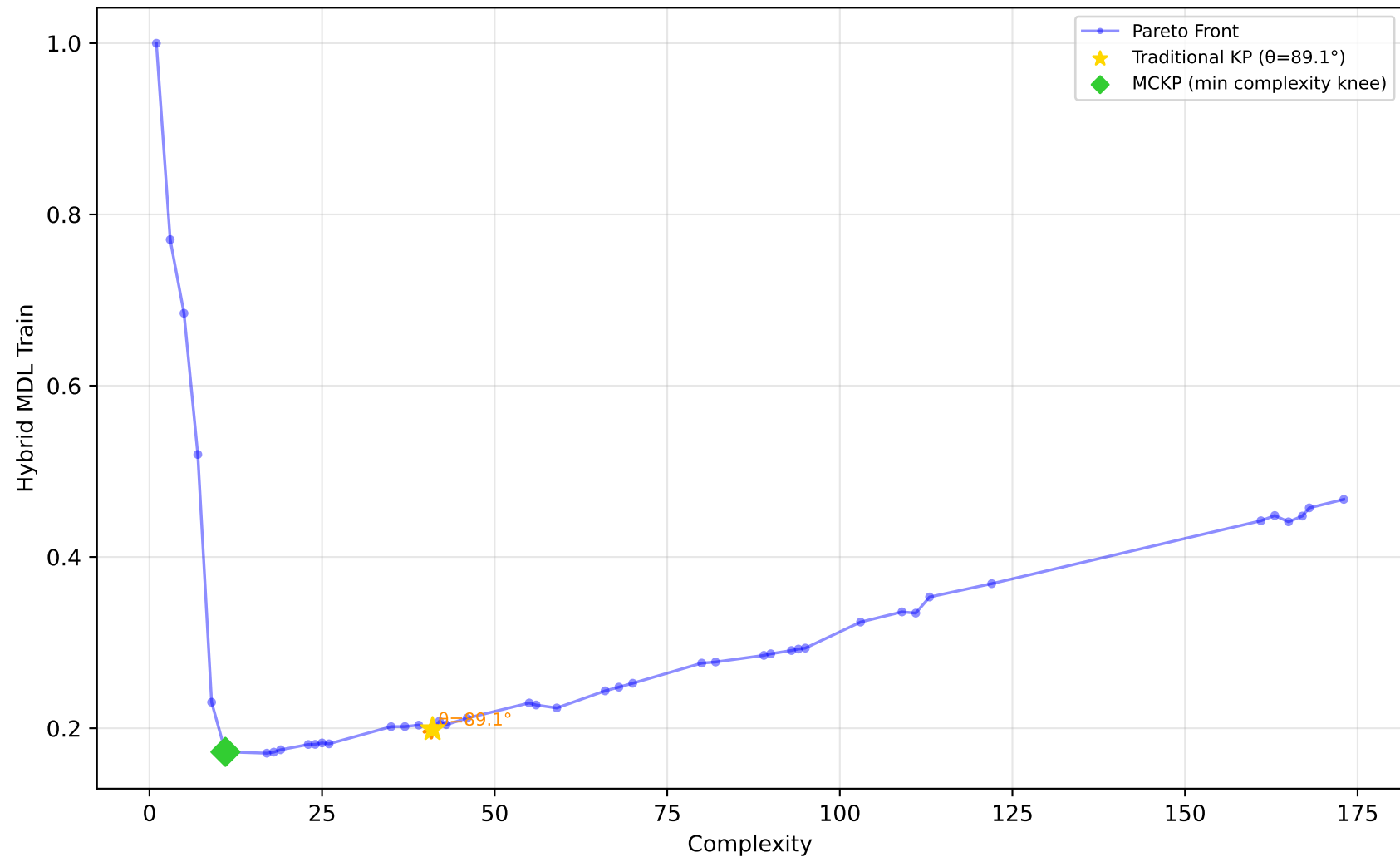
529_pollen - Run 15 - MVP - Hybrid MDL Train \lambda_1=0.90, \lambda_2=0.00, \lambda_3=0.00 | Difficulty: 1.00 | Method: hmr
