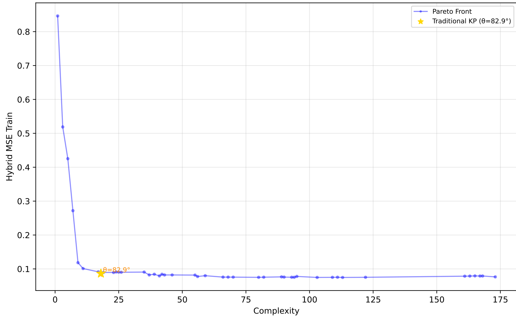
529_pollen - Run 15 - MVP - Hybrid MSE Train \lambda_1=0.00, \lambda_2=1.00, \lambda_3=0.80 | Difficulty: 1.00 | Method: hmr
