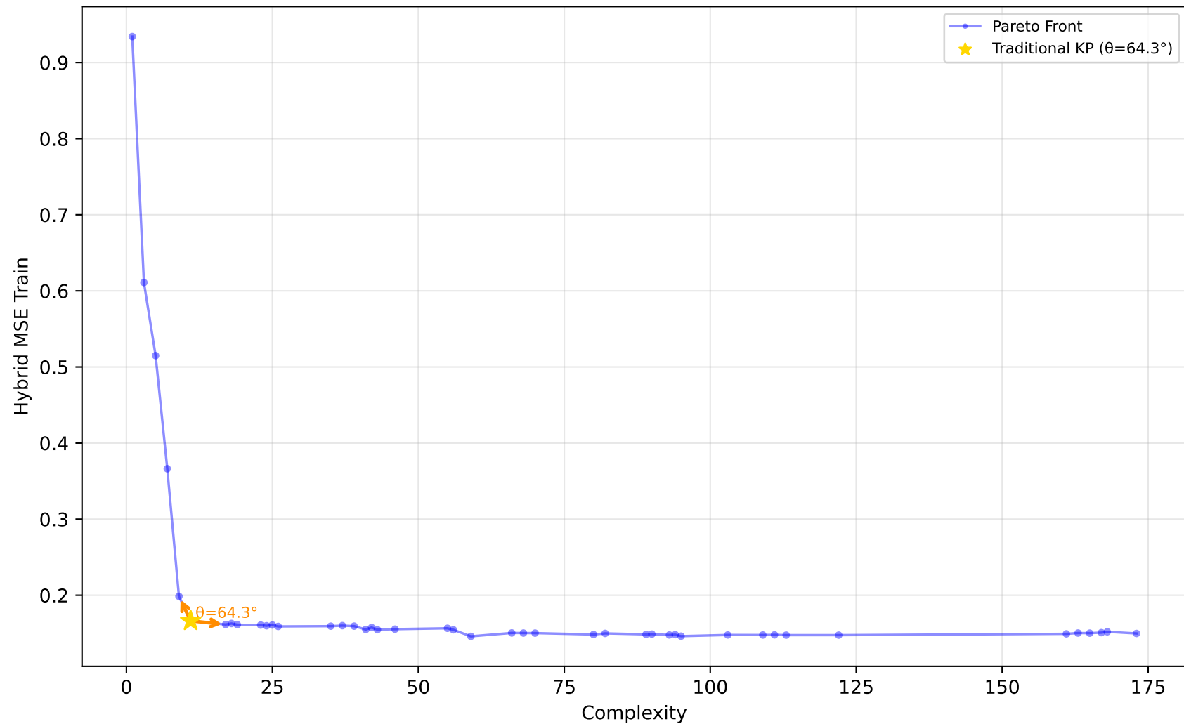
529_pollen - Run 15 - MVP - Hybrid MSE Train \lambda_1=0.90, \lambda_2=0.00, \lambda_3=0.00 | Difficulty: 1.00 | Method: hmr
