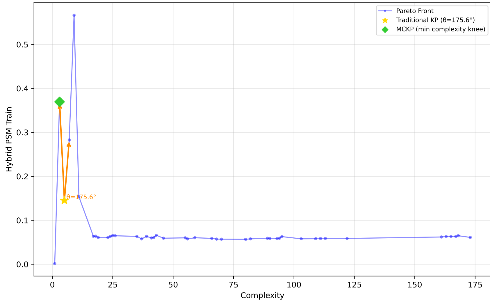
529_pollen - Run 15 - MVP - Hybrid PSM Train \lambda_1=0.00, \lambda_2=1.00, \lambda_3=0.80 | Difficulty: 1.00 | Method: hmr
