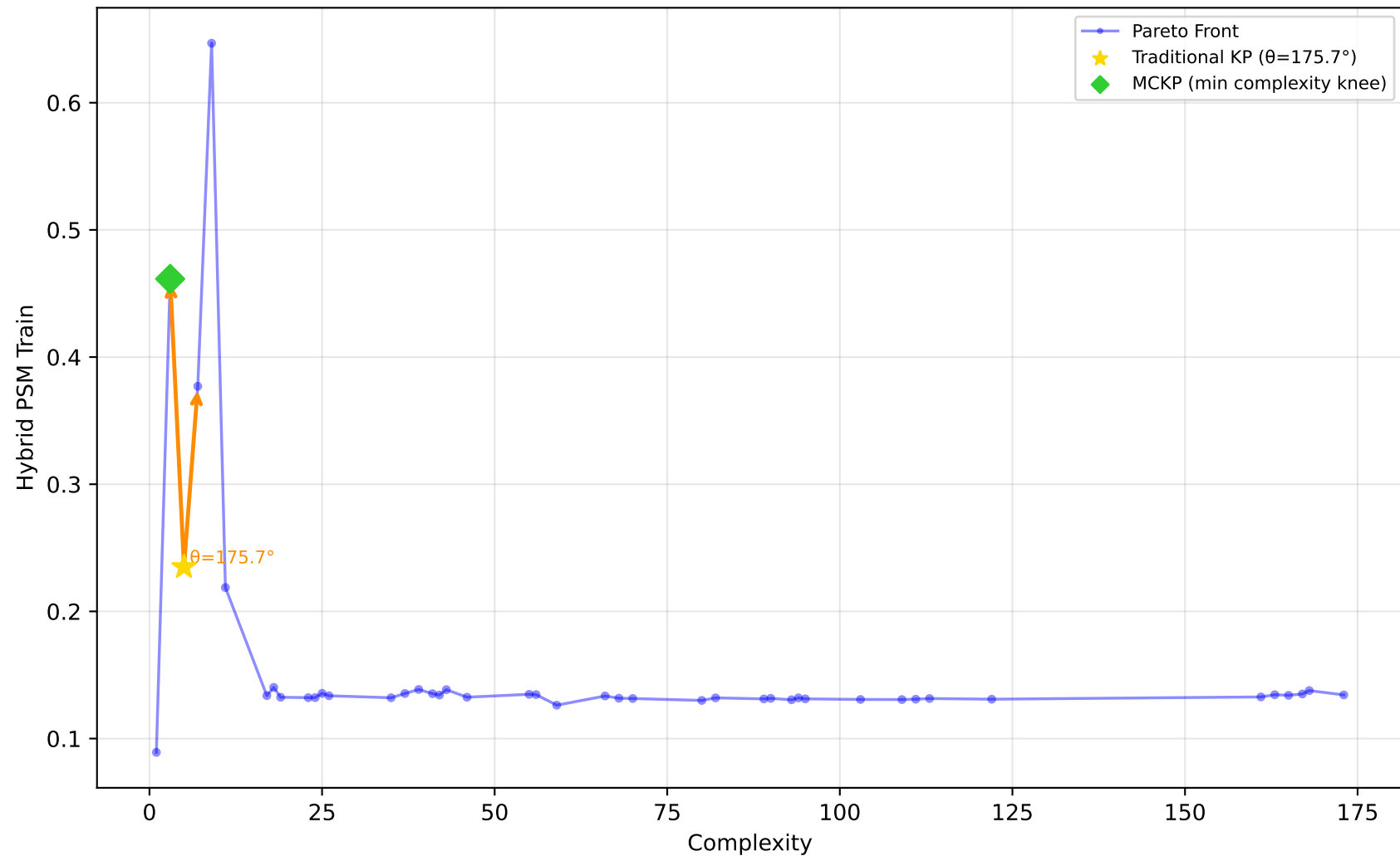
529_pollen - Run 15 - MVP - Hybrid PSM Train \lambda_1=0.90, \lambda_2=0.00, \lambda_3=0.00 | Difficulty: 1.00 | Method: hmr
