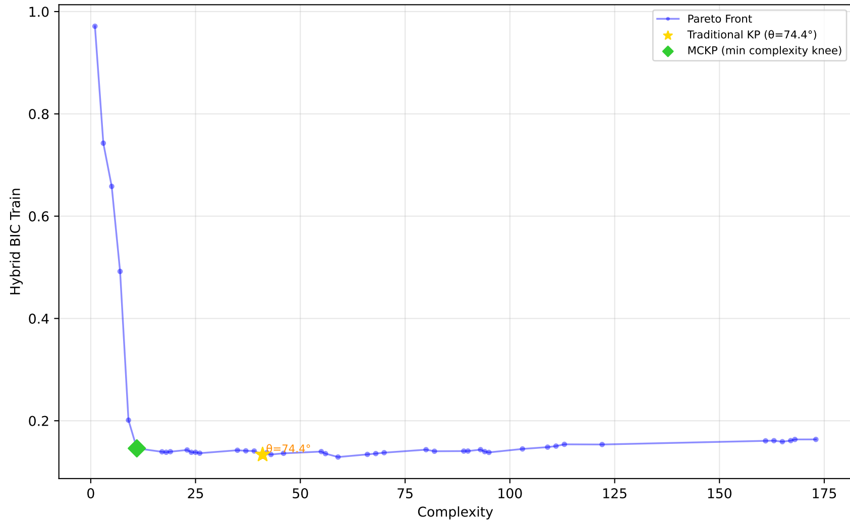
529_pollen - Run 15 - SVP - Hybrid BIC Train \lambda_1=0.60, \lambda_2=0.40, \lambda_3=1.00 | Difficulty: 1.00 | Method: hmr
