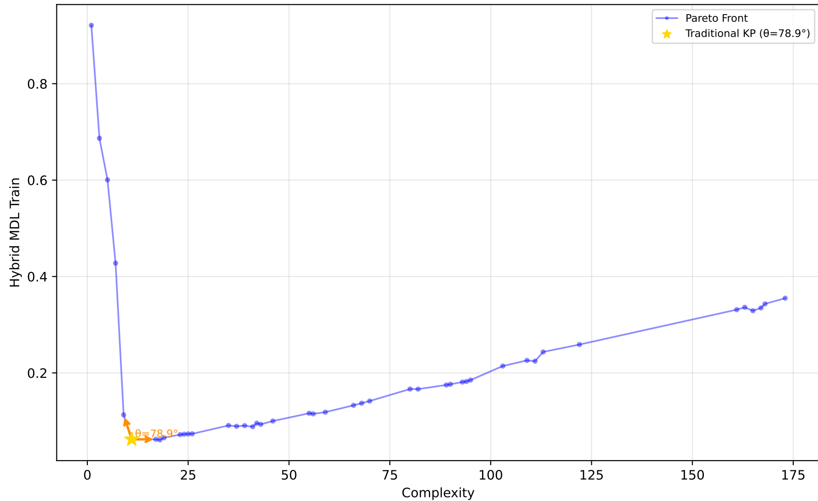
529_pollen - Run 15 - SVP - Hybrid MDL Train \lambda_1=0.10, \lambda_2=0.80, \lambda_3=0.30 | Difficulty: 1.00 | Method: hmr
