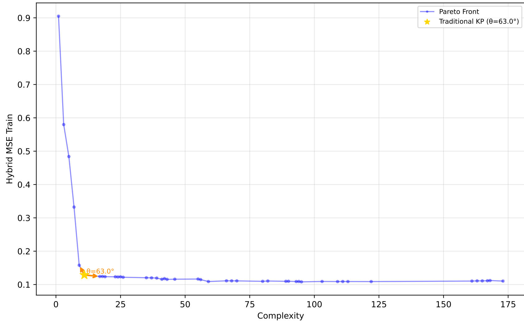
529_pollen - Run 15 - SVP - Hybrid MSE Train \lambda_1=0.60, \lambda_2=0.40, \lambda_3=1.00 | Difficulty: 1.00 | Method: hmr
