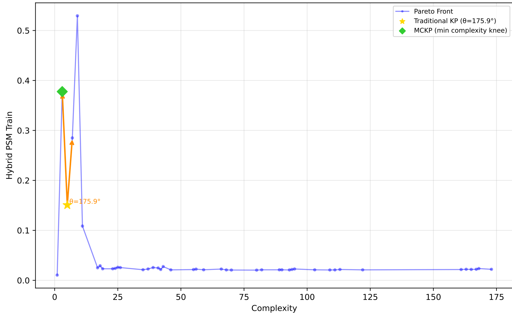
529_pollen - Run 15 - SVP - Hybrid PSM Train \lambda_1=0.10, \lambda_2=0.80, \lambda_3=0.30 | Difficulty: 1.00 | Method: hmr
