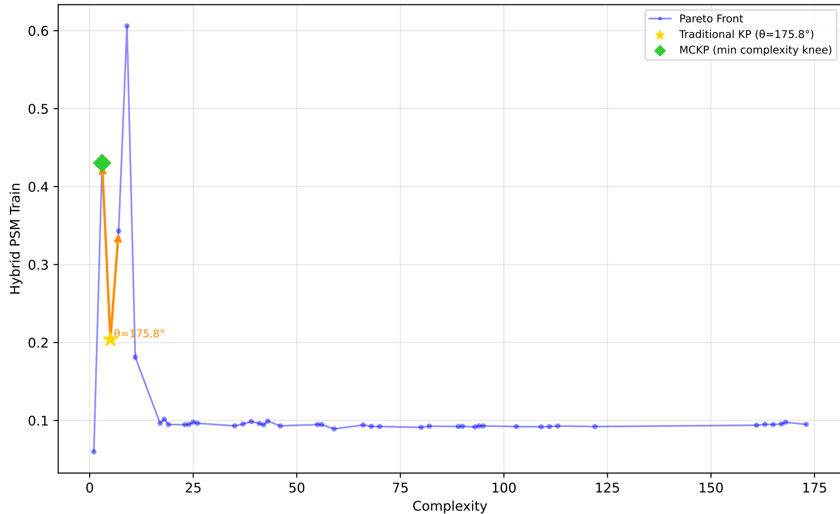
529_pollen - Run 15 - SVP - Hybrid PSM Train \lambda_1=0.60, \lambda_2=0.40, \lambda_3=1.00 | Difficulty: 1.00 | Method: hmr
