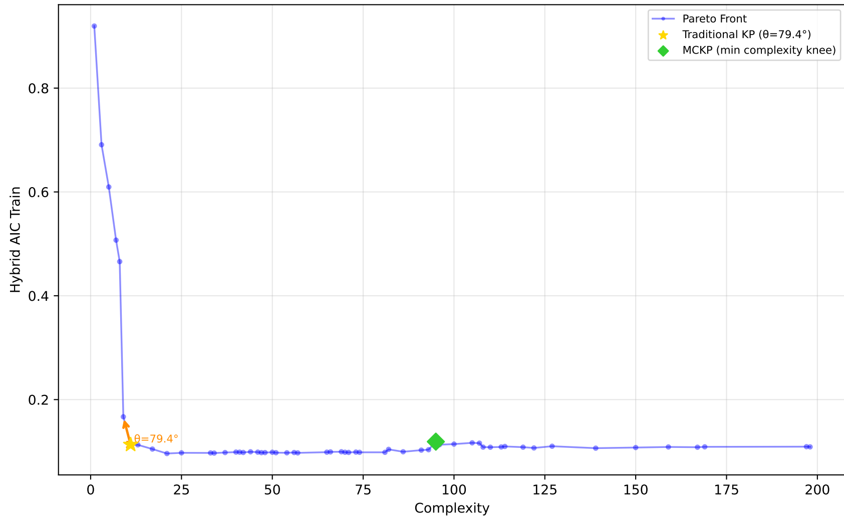
529_pollen - Run 16 - MVP - Hybrid AIC Train \lambda_1=0.00, \lambda_2=1.00, \lambda_3=0.80 | Difficulty: 1.00 | Method: hmr
