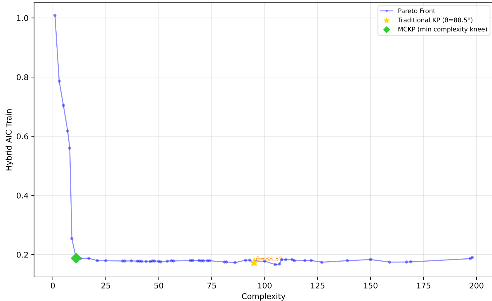
529_pollen - Run 16 - MVP - Hybrid AIC Train \lambda_1=0.90, \lambda_2=0.00, \lambda_3=0.00 | Difficulty: 1.00 | Method: hmr
