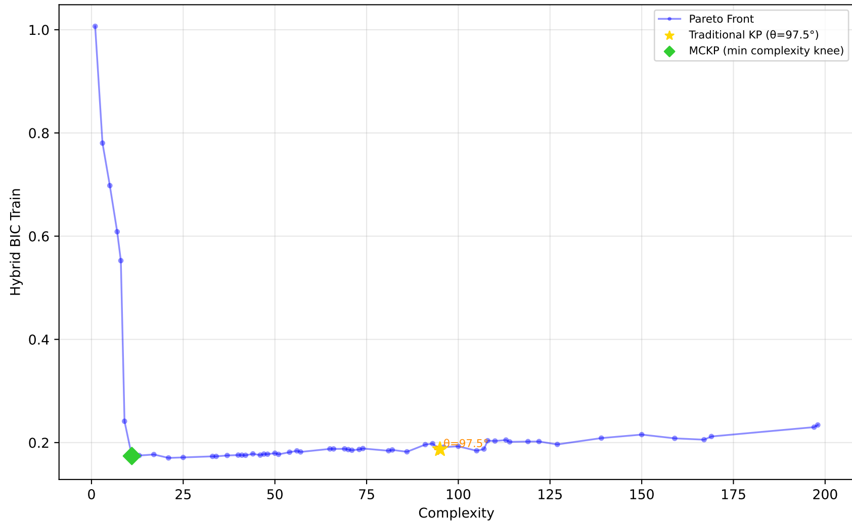
529_pollen - Run 16 - MVP - Hybrid BIC Train \lambda_1=0.90, \lambda_2=0.00, \lambda_3=0.00 | Difficulty: 1.00 | Method: hmr
