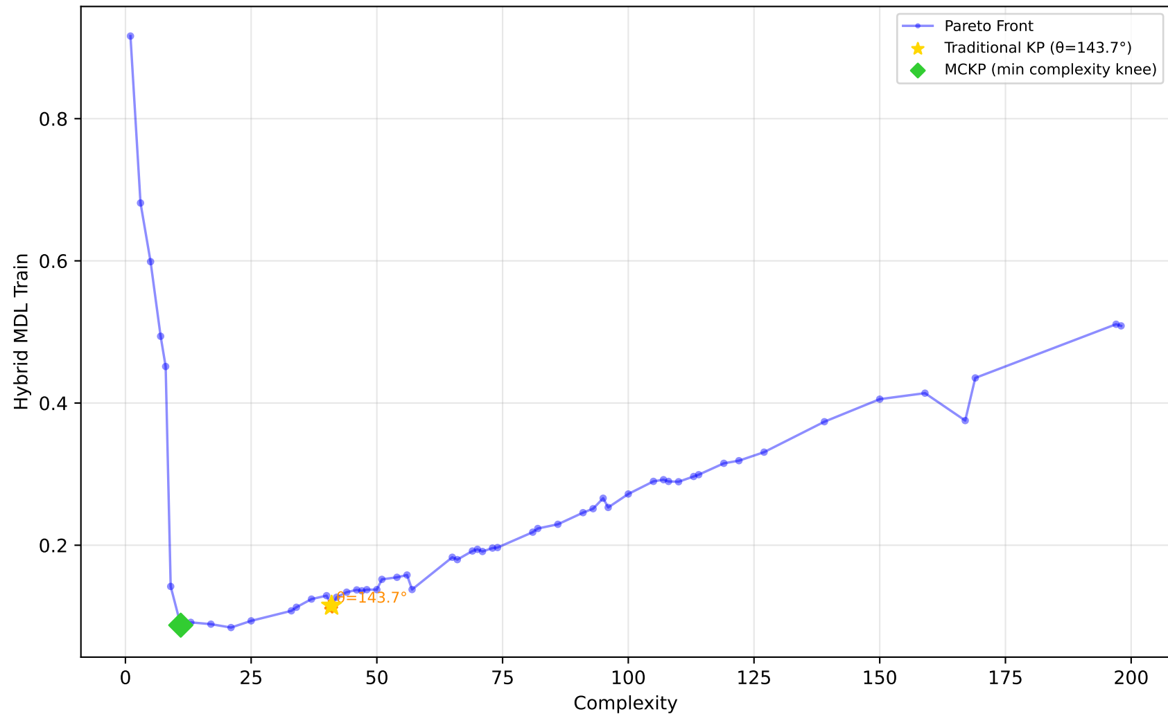
529_pollen - Run 16 - MVP - Hybrid MDL Train \lambda_1=0.00 , \lambda_2=1.00 , \lambda_3=0.80 | Difficulty: 1.00 | Method: hmr
