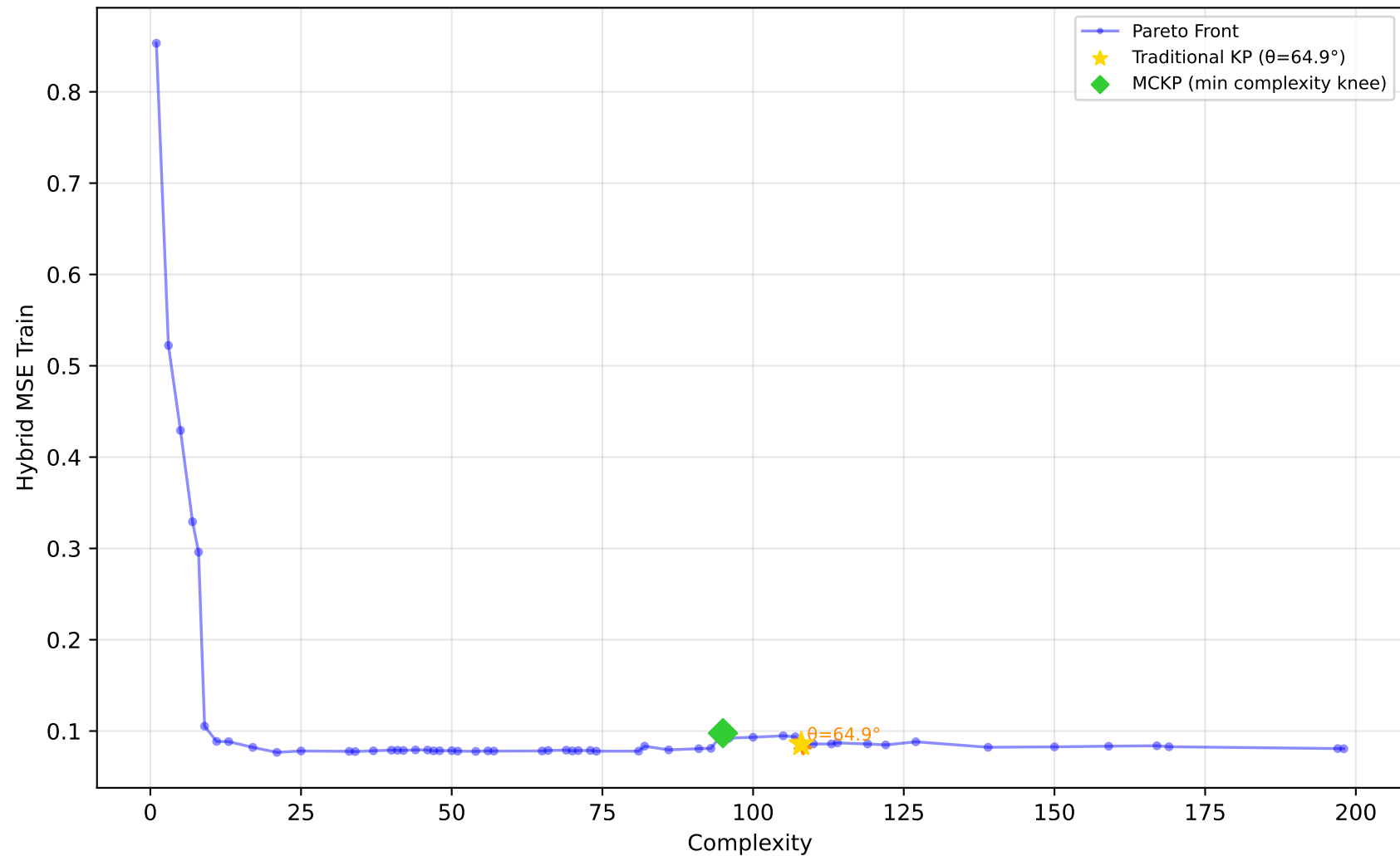
529_pollen - Run 16 - MVP - Hybrid MSE Train \lambda_1=0.00, \lambda_2=1.00, \lambda_3=0.80 | Difficulty: 1.00 | Method: hmr
