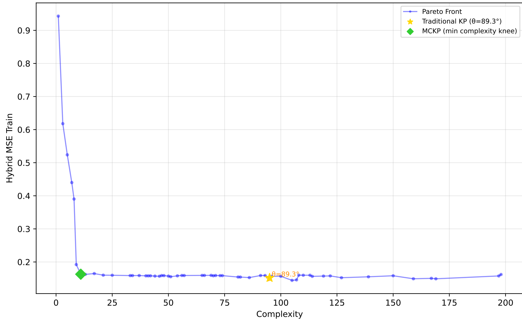
529_pollen - Run 16 - MVP - Hybrid MSE Train \lambda_1=0.90, \lambda_2=0.00, \lambda_3=0.00 | Difficulty: 1.00 | Method: hmr
