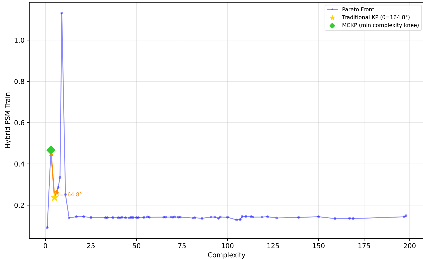
529_pollen - Run 16 - MVP - Hybrid PSM Train \lambda_1=0.90, \lambda_2=0.00, \lambda_3=0.00 | Difficulty: 1.00 | Method: hmr
