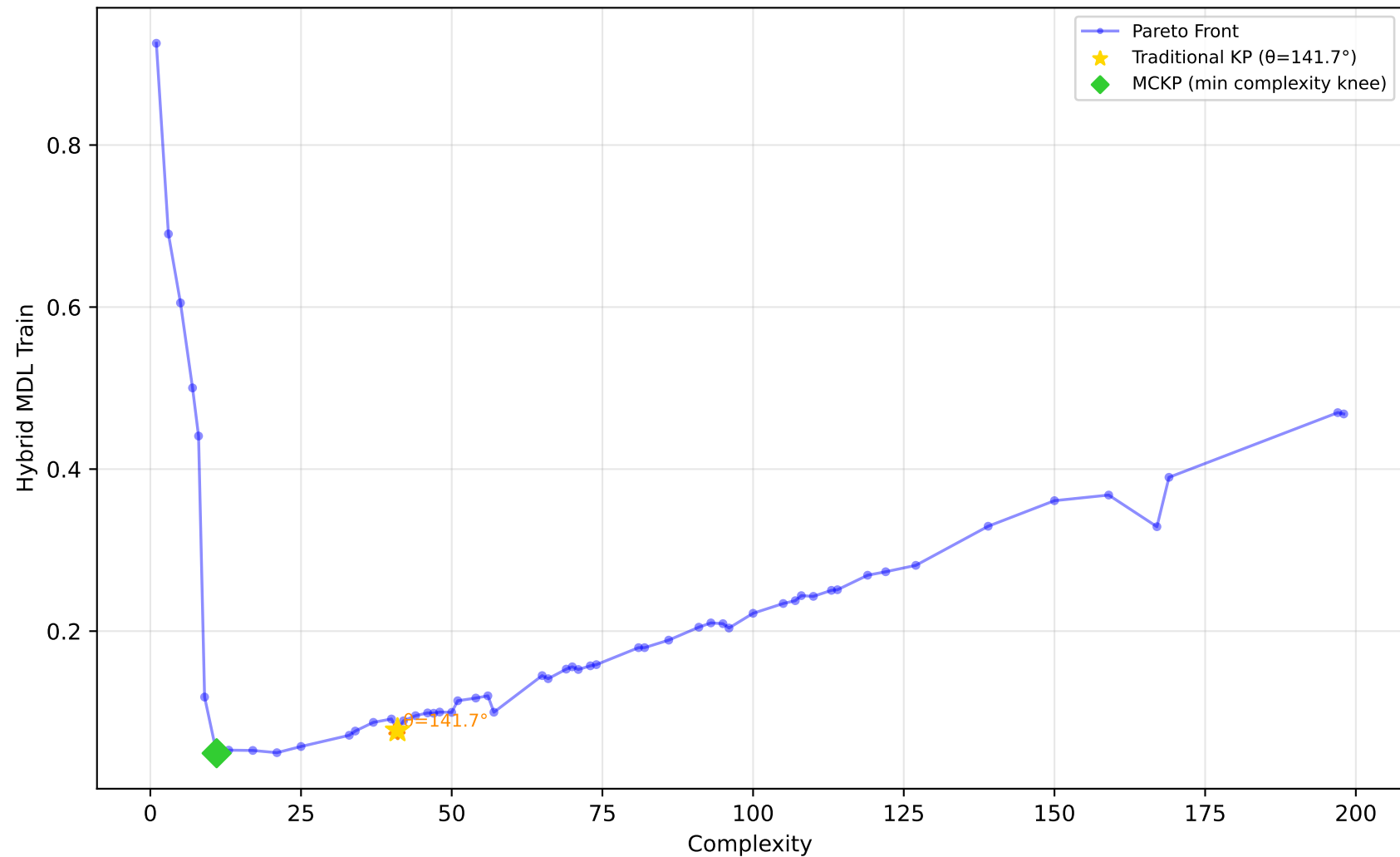
529_pollen - Run 16 - SVP - Hybrid MDL Train \lambda_1=0.10, \lambda_2=0.80, \lambda_3=0.30 | Difficulty: 1.00 | Method: hmr
