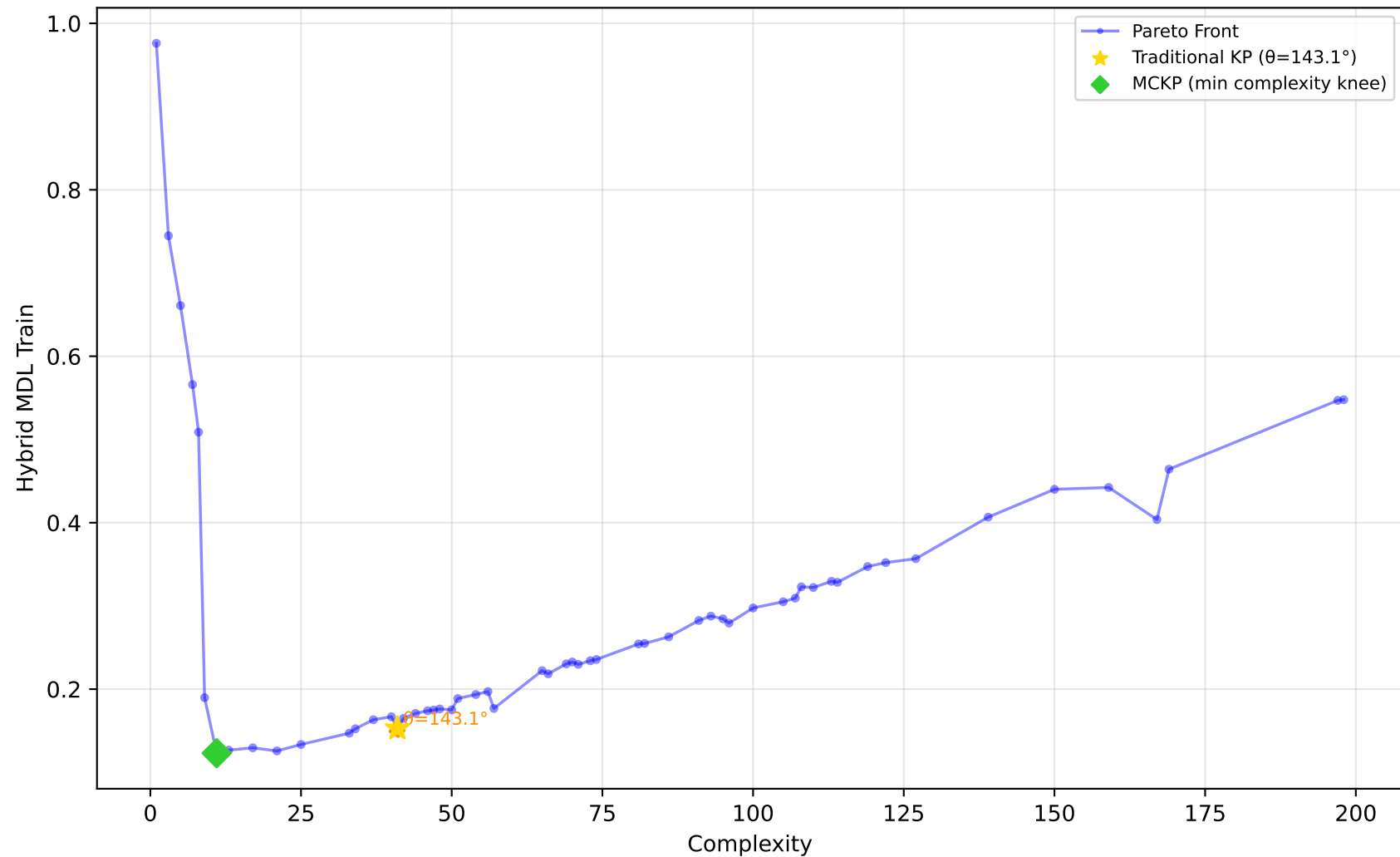
529_pollen - Run 16 - SVP - Hybrid MDL Train \lambda_1=0.60, \lambda_2=0.40, \lambda_3=1.00 | Difficulty: 1.00 | Method: hmr
