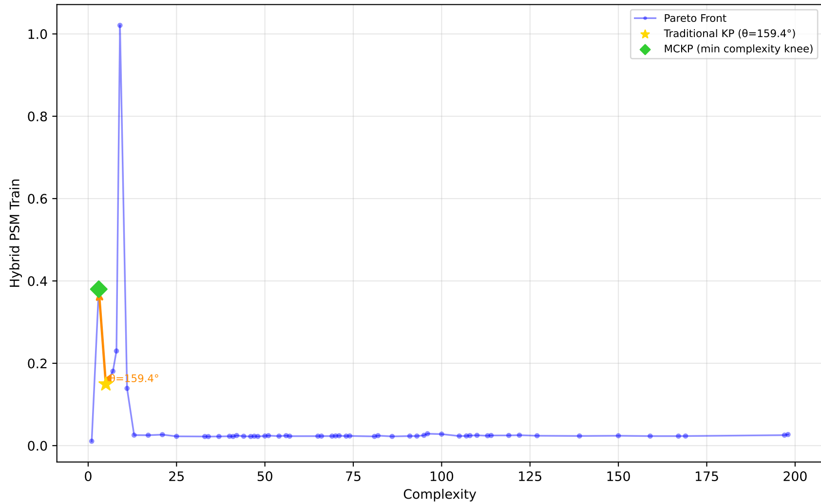
529_pollen - Run 16 - SVP - Hybrid PSM Train \lambda_1=0.10, \lambda_2=0.80, \lambda_3=0.30 | Difficulty: 1.00 | Method: hmr
