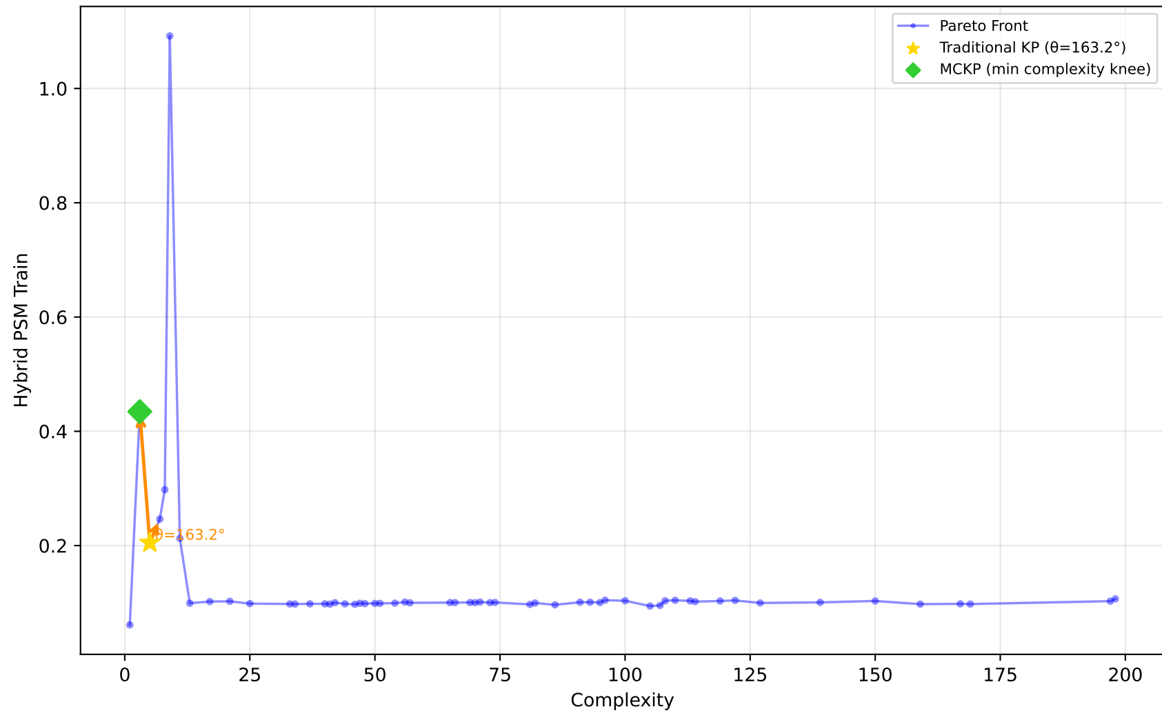
529_pollen - Run 16 - SVP - Hybrid PSM Train \lambda_1=0.60, \lambda_2=0.40, \lambda_3=1.00 | Difficulty: 1.00 | Method: hmr
