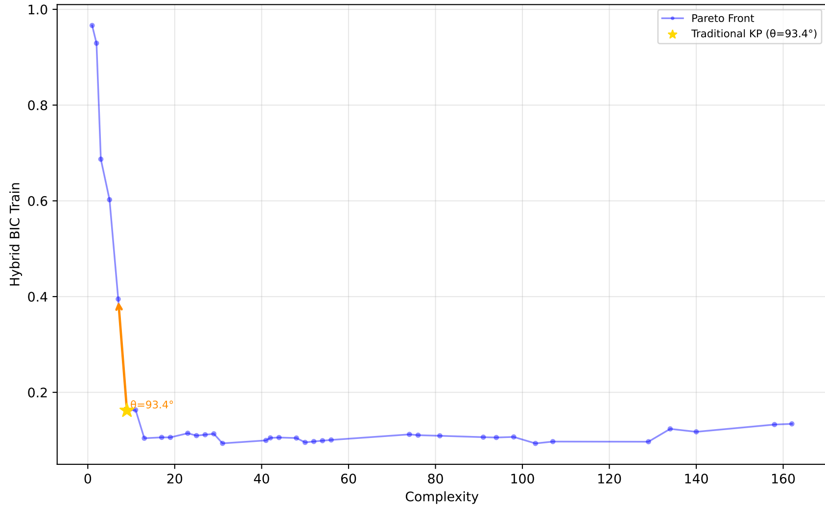
529_pollen - Run 17 - MVP - Hybrid BIC Train \lambda_1=0.00 , \lambda_2=1.00 , \lambda_3=0.80 | Difficulty: 1.00 | Method: hmr
