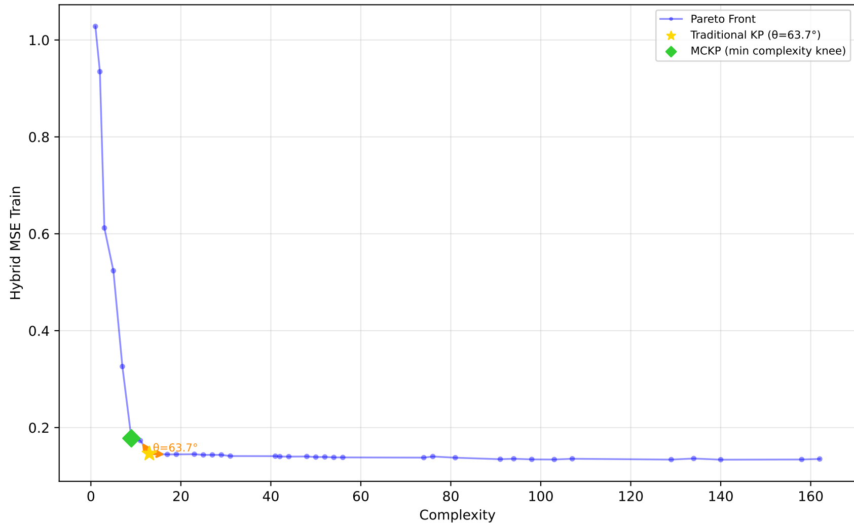
529_pollen - Run 17 - MVP - Hybrid MSE Train \lambda_1=0.90, \lambda_2=0.00, \lambda_3=0.00 | Difficulty: 1.00 | Method: hmr
