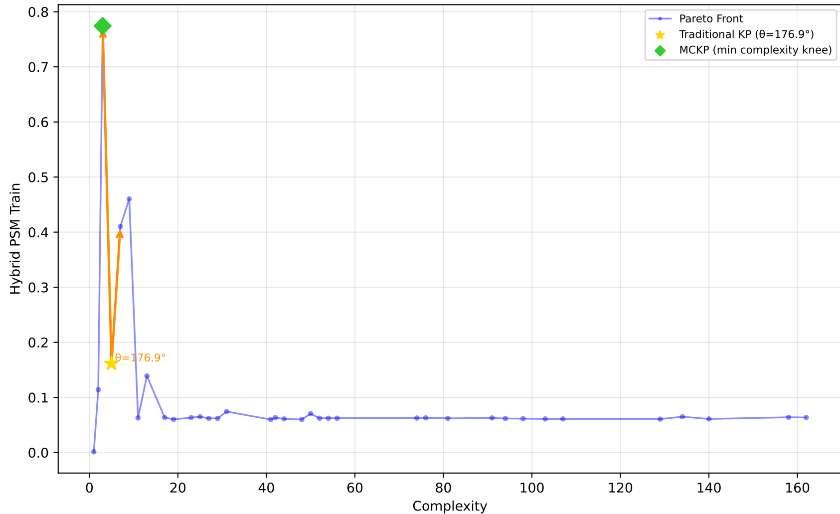
529_pollen - Run 17 - MVP - Hybrid PSM Train \lambda_1=0.00, \lambda_2=1.00, \lambda_3=0.80 | Difficulty: 1.00 | Method: hmr
