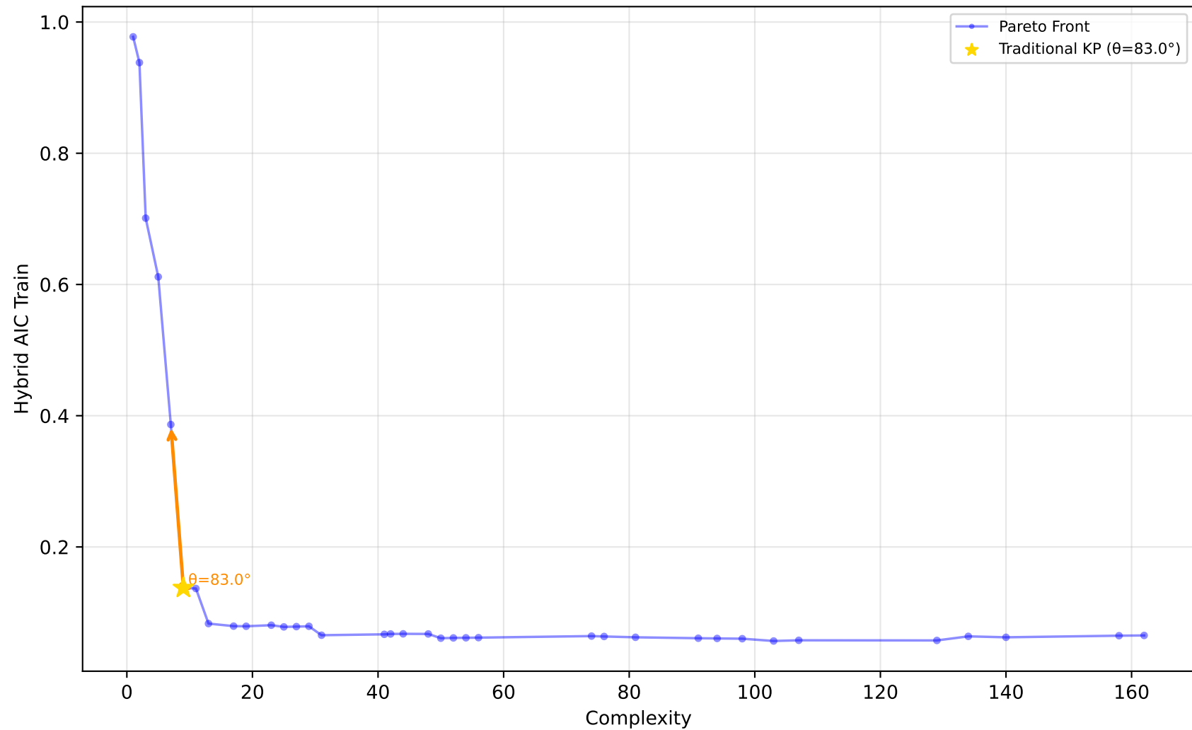
529_pollen - Run 17 - SVP - Hybrid AIC Train \lambda_1=0.10, \lambda_2=0.80, \lambda_3=0.30 | Difficulty: 1.00 | Method: hmr
