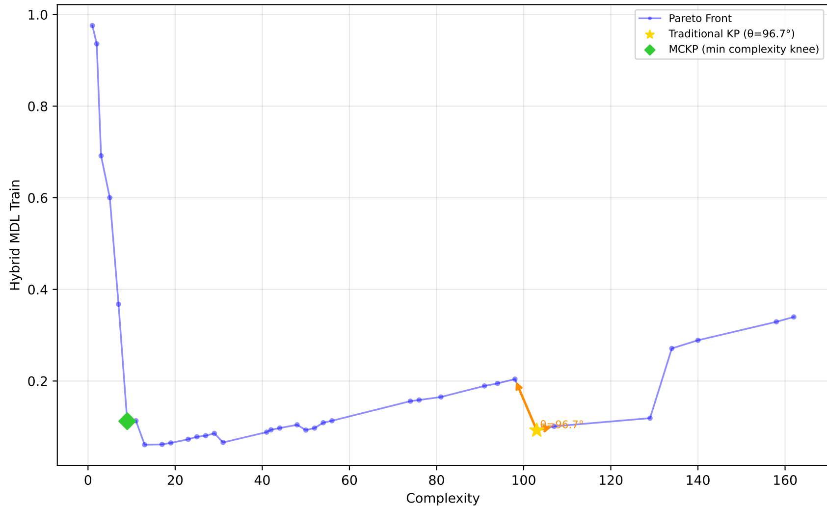
529_pollen - Run 17 - SVP - Hybrid MDL Train \lambda_1=0.10, \lambda_2=0.80, \lambda_3=0.30 | Difficulty: 1.00 | Method: hmr
