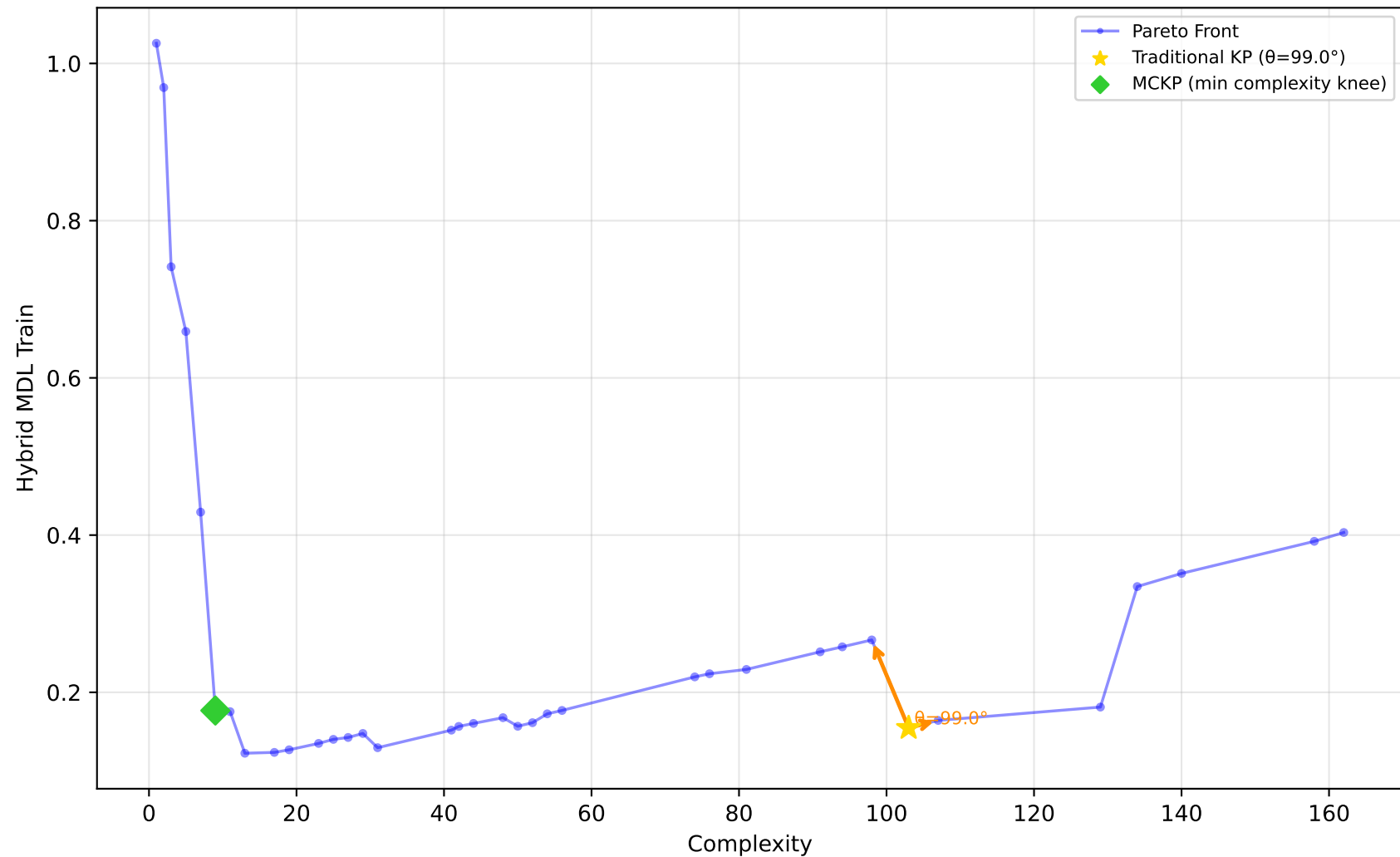
529_pollen - Run 17 - SVP - Hybrid MDL Train \lambda_1=0.60, \lambda_2=0.40, \lambda_3=1.00 | Difficulty: 1.00 | Method: hmr
