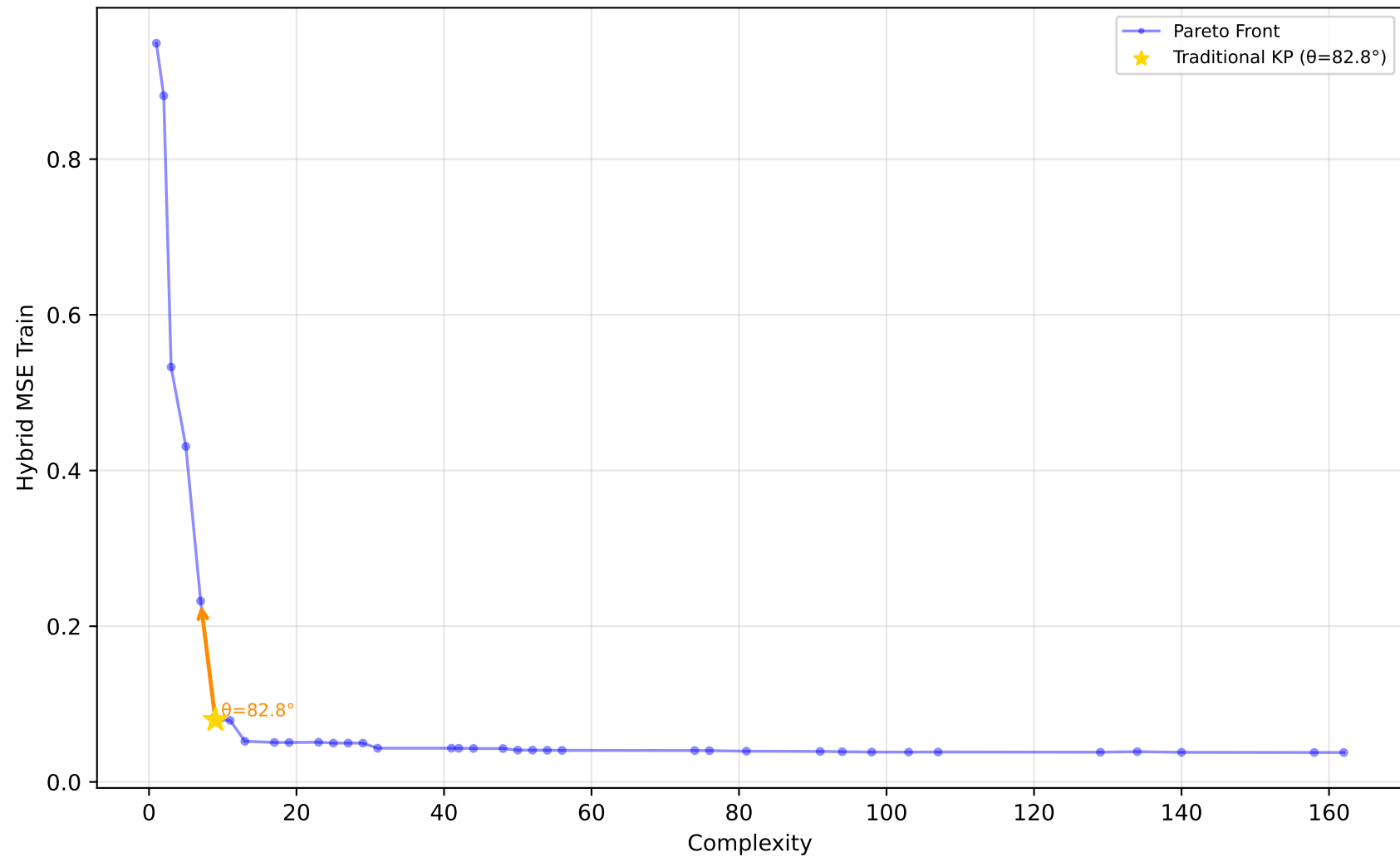
529_pollen - Run 17 - SVP - Hybrid MSE Train \lambda_1=0.10, \lambda_2=0.80, \lambda_3=0.30 | Difficulty: 1.00 | Method: hmr
