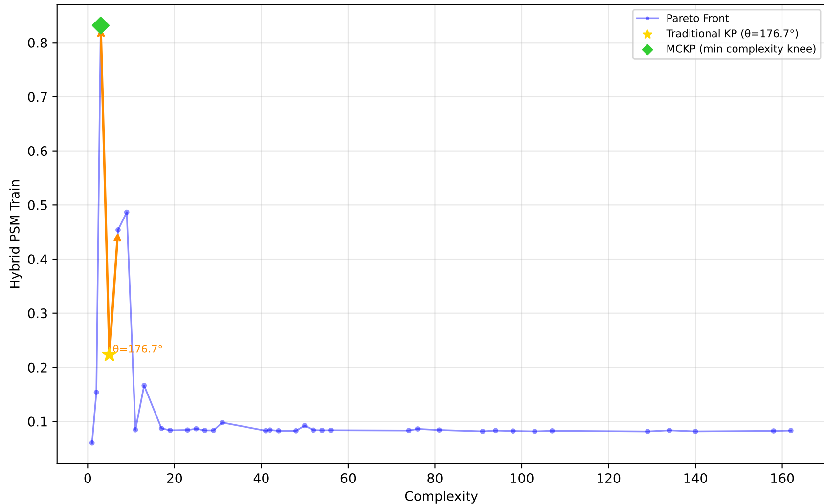
529_pollen - Run 17 - SVP - Hybrid PSM Train \lambda_1=0.60, \lambda_2=0.40, \lambda_3=1.00 | Difficulty: 1.00 | Method: hmr
