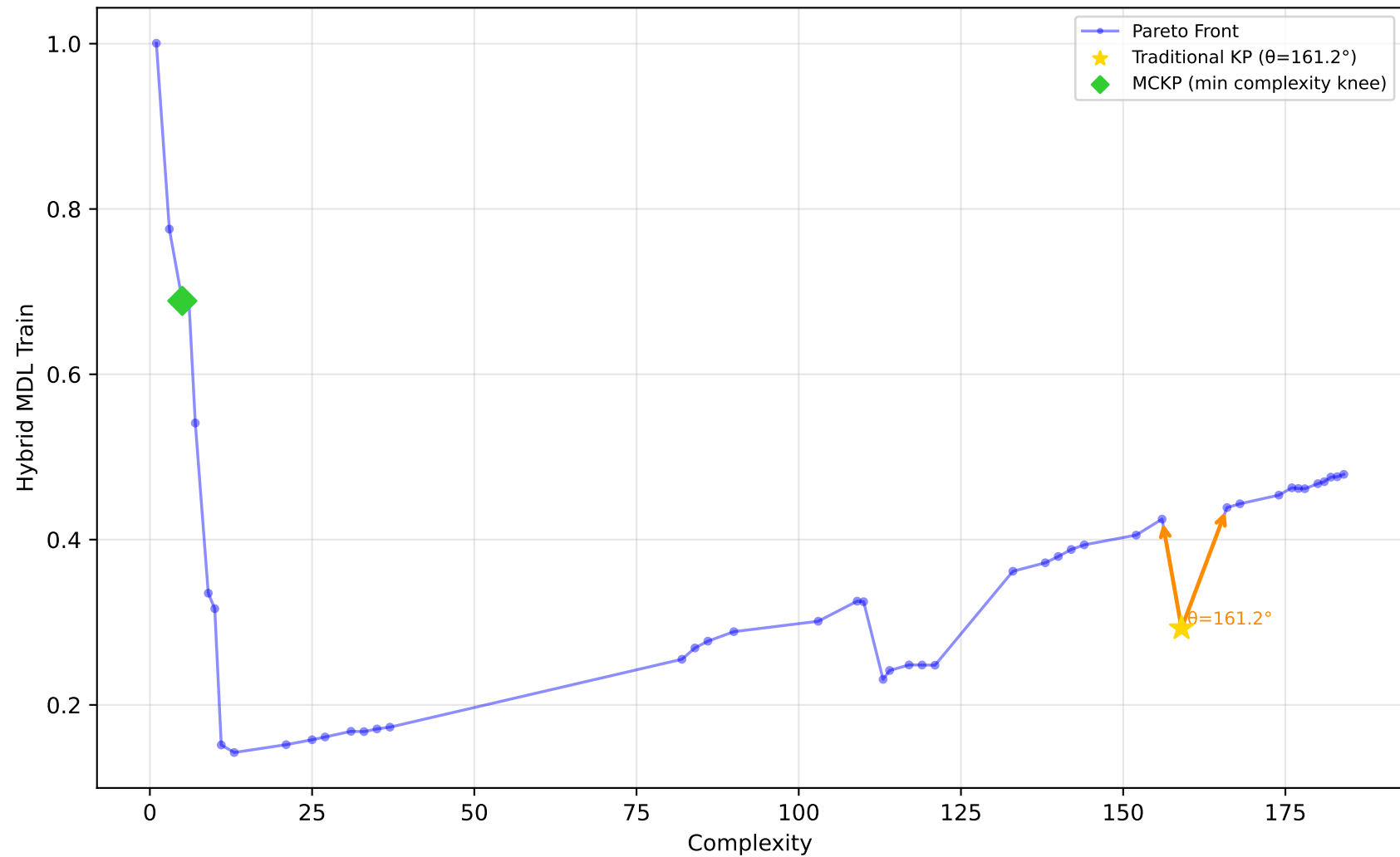
529_pollen - Run 18 - MVP - Hybrid MDL Train \lambda_1=0.90, \lambda_2=0.00, \lambda_3=0.00 | Difficulty: 1.00 | Method: hmr
