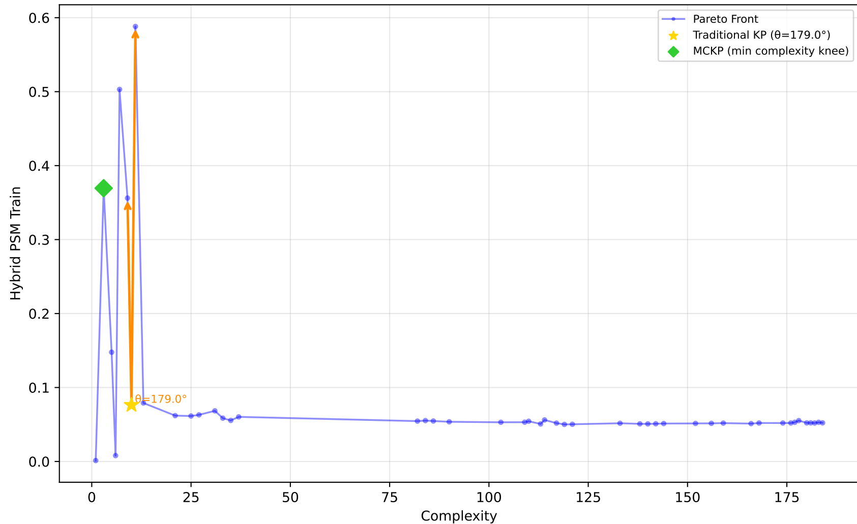
529_pollen - Run 18 - MVP - Hybrid PSM Train \lambda_1=0.00, \lambda_2=1.00, \lambda_3=0.80 | Difficulty: 1.00 | Method: hmr
